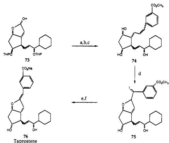
Scheme 16 a
