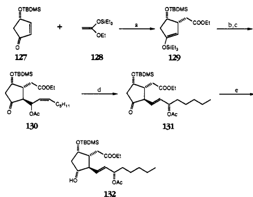
Scheme 32 a
