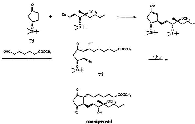
Scheme 20 a
