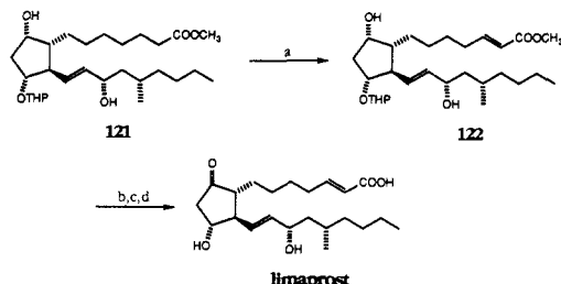
Scheme 30 a
