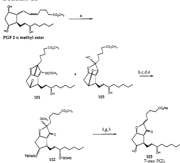
Scheme 22 a
