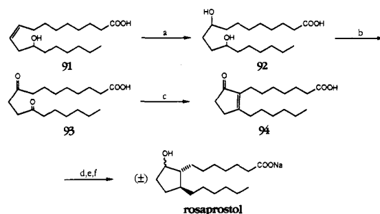
Scheme 25*
