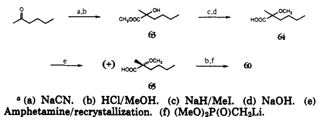
Scheme 18 a
