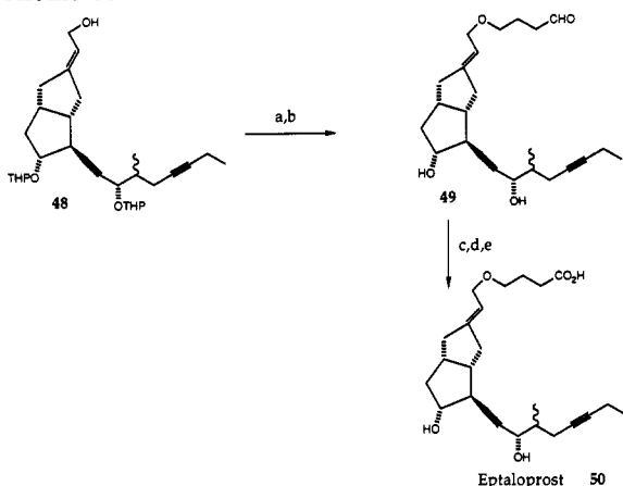
Scheme 11 a
