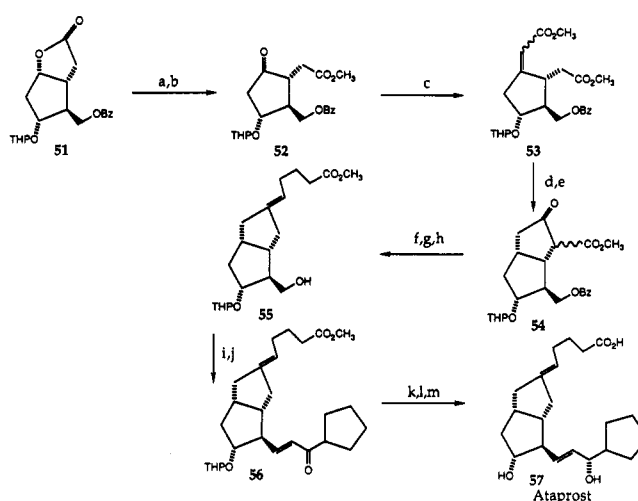
Scheme 12 a
