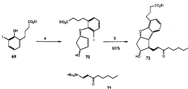
Scheme 15 a
