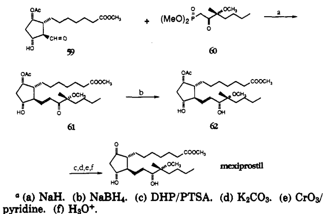
Scheme 17 a
