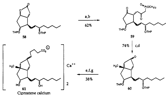
Scheme 13 a
