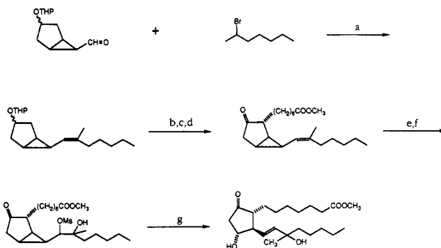
Scheme 2 a
