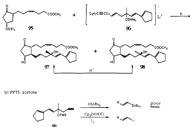
Scheme 26
