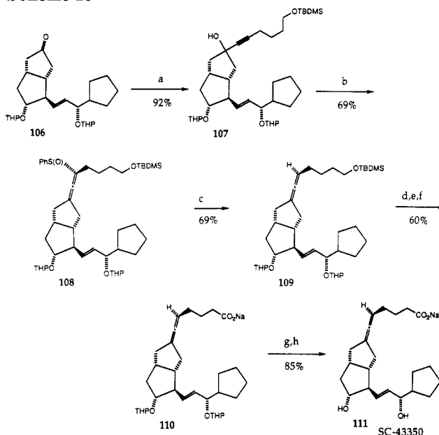
Scheme 23 a
