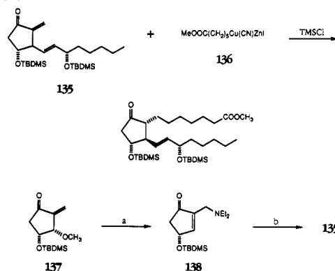
Scheme 34 a
