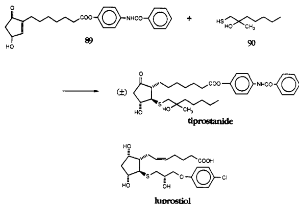
Scheme 24
