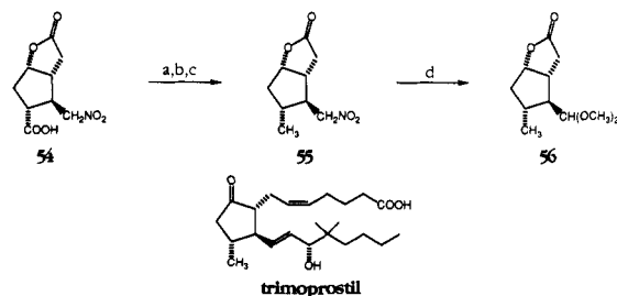
Scheme 15 a
