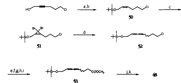
Scheme 14 a
