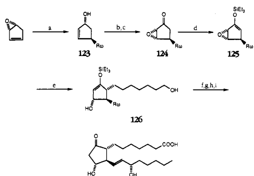
Scheme 31 a
