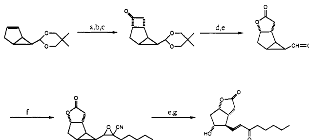
Scheme 3 a
