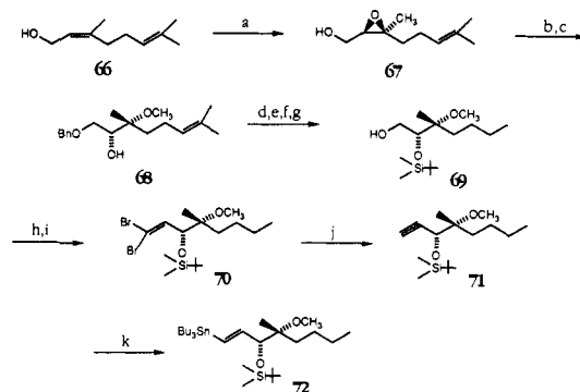
Scheme 19 a
