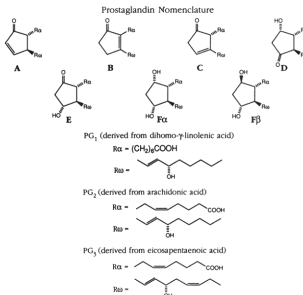
Figure 2. Prostaglandin nomenclature.
